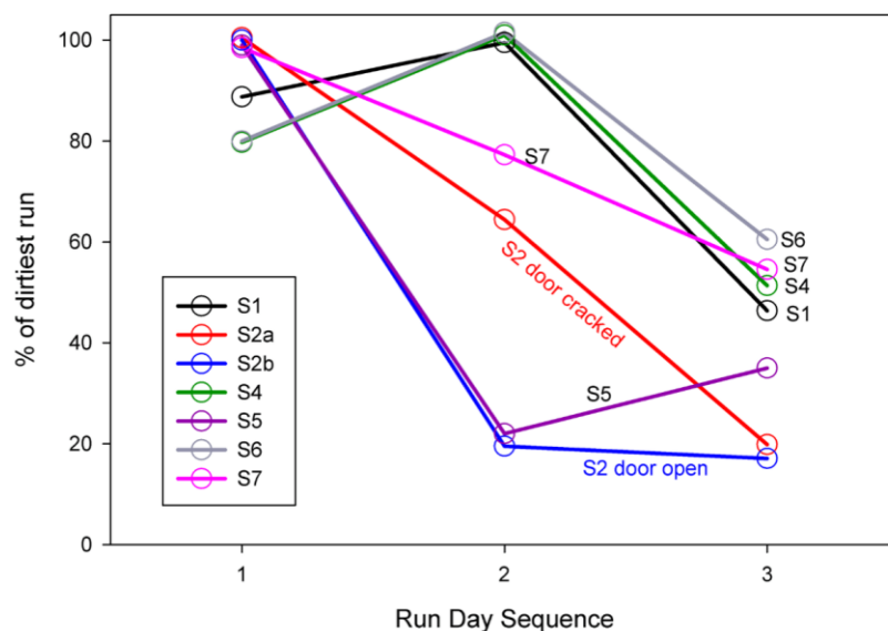
Figure 13. Emission Outcomes Replicate Testing
